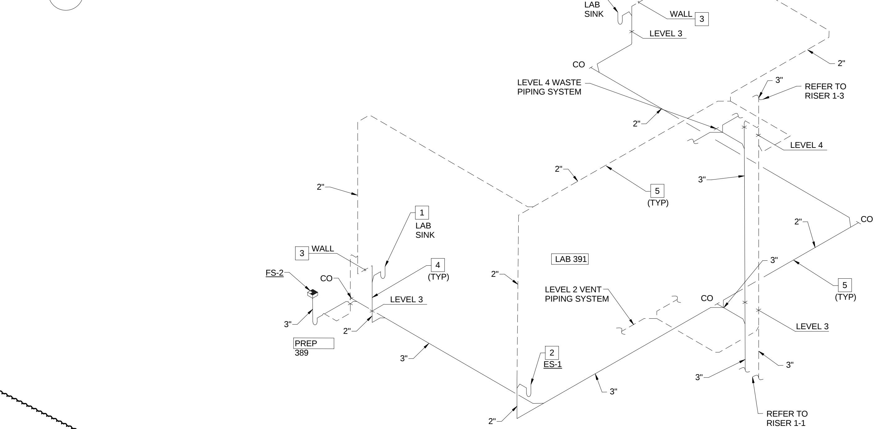
1-2 SANITARY WASTE AND VENT RISER - PREP 389 AND LAB 391
