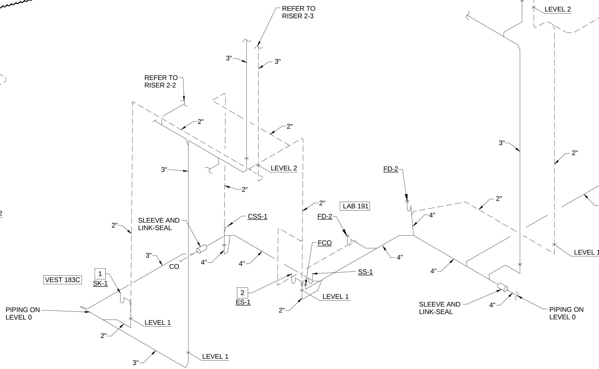
2-1 SANITARY WASTE AND VENT RISER - VESTIBULE 183C AND LAB 191
